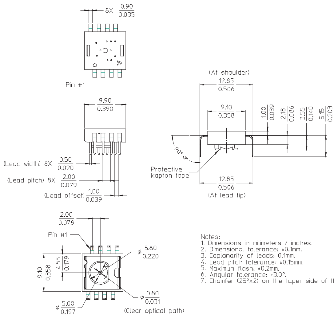
Figure 2. Package outline drawing
